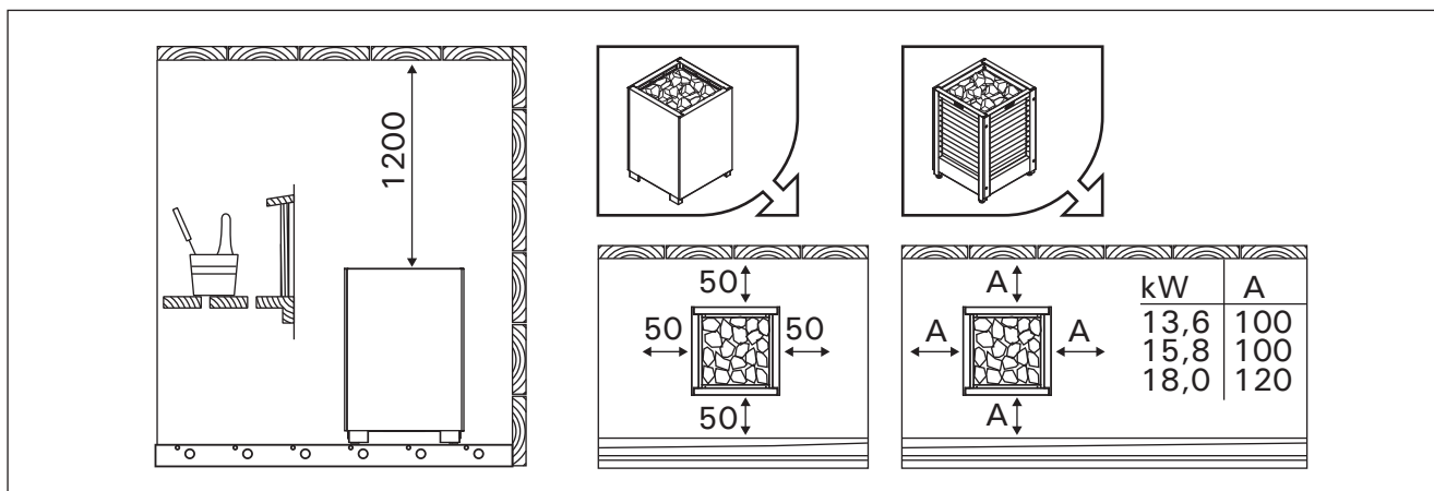
Figure 4. Minimum safety distances (all dimensions in millimeters)
